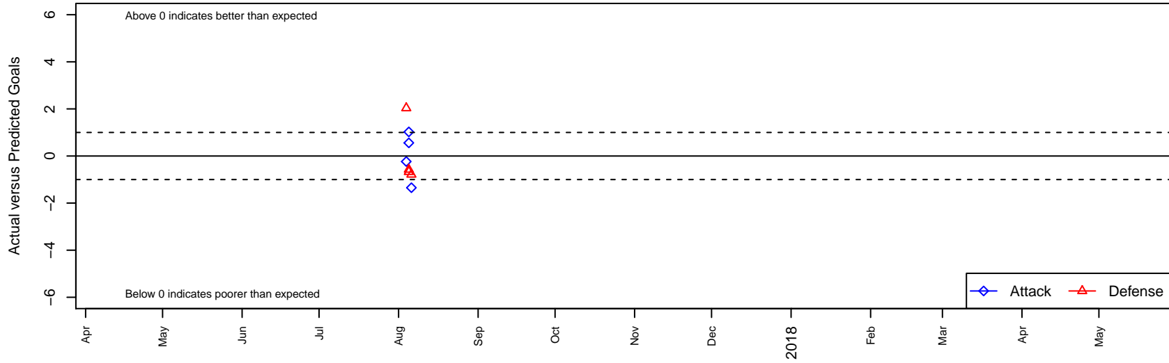
San Diego Machine SC B99 Dots are actual minus expected GF (blue circles) and GA (red triangles). Blue line is smoothed change in attack strength. Red is smoothed change in defense strength.
